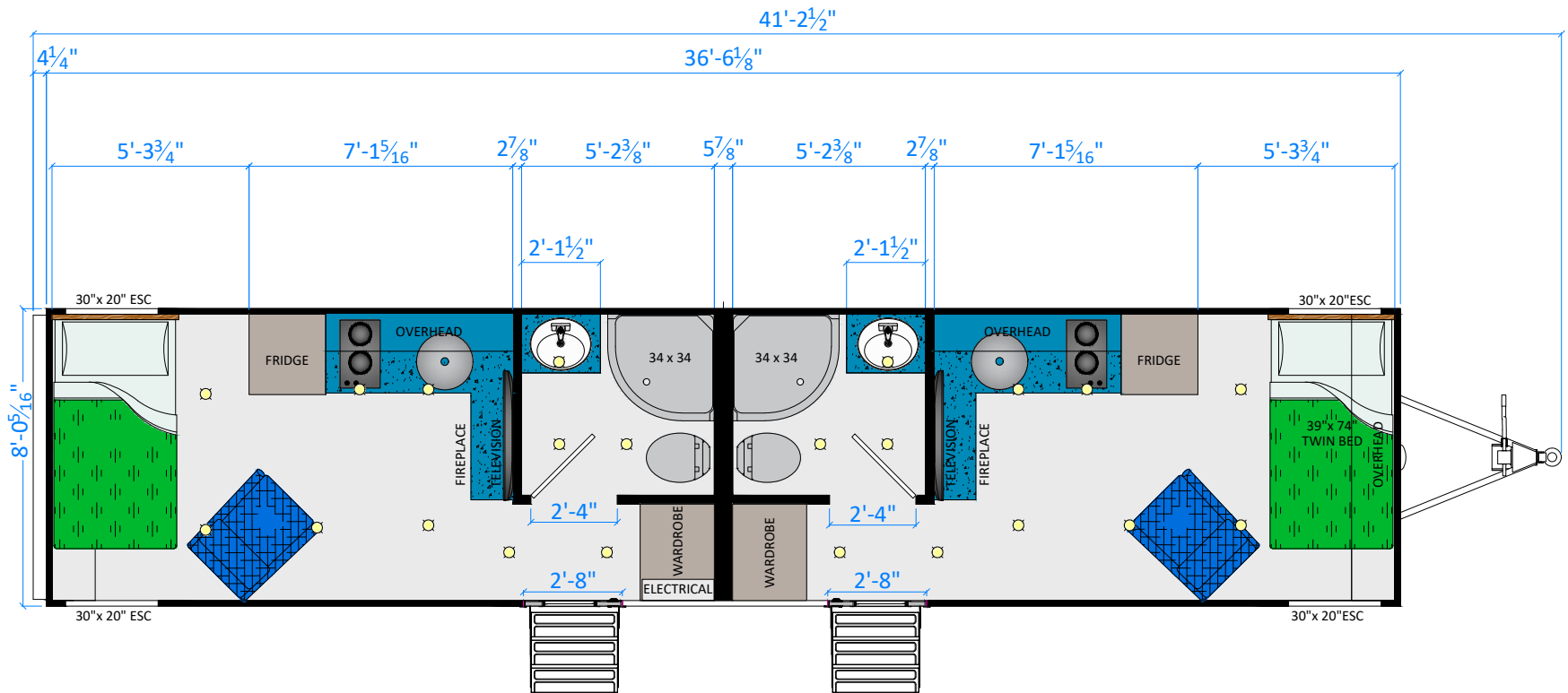
CITATION 2 PERSON HOUSING TRAILER (CDN) 293 SQ.FT.
