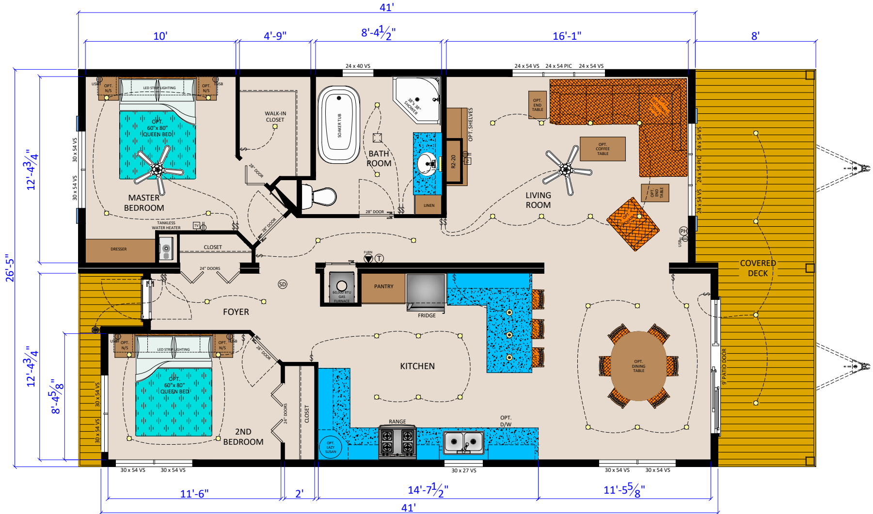
RICHDALE 21 (R4113+R4113) (540 SQ.FT.)+(529 SQ.FT.)
