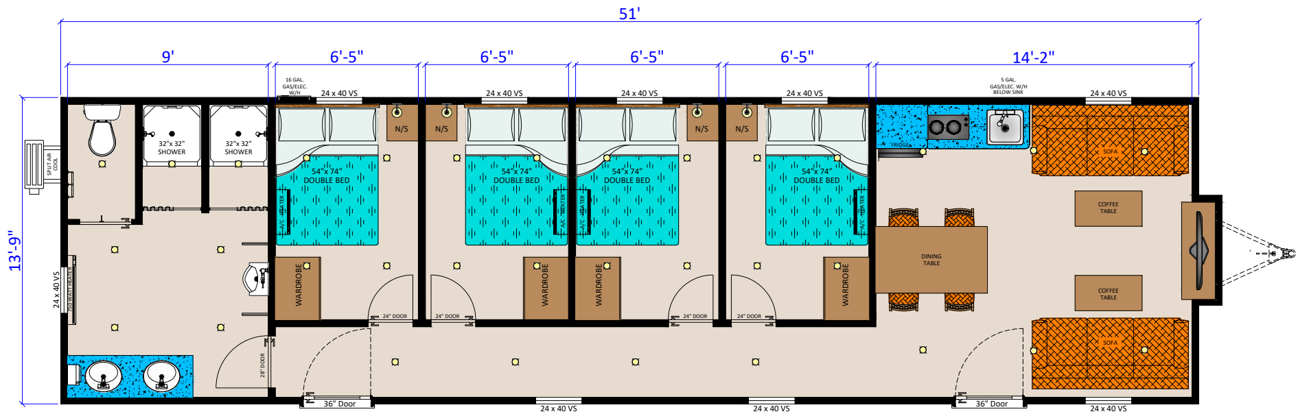
WORKFORCE 4 PERSON COMBO WF5114 - 4 COMBO (722.8 SQ. FT.) STAFF HOUSING TRAILER
