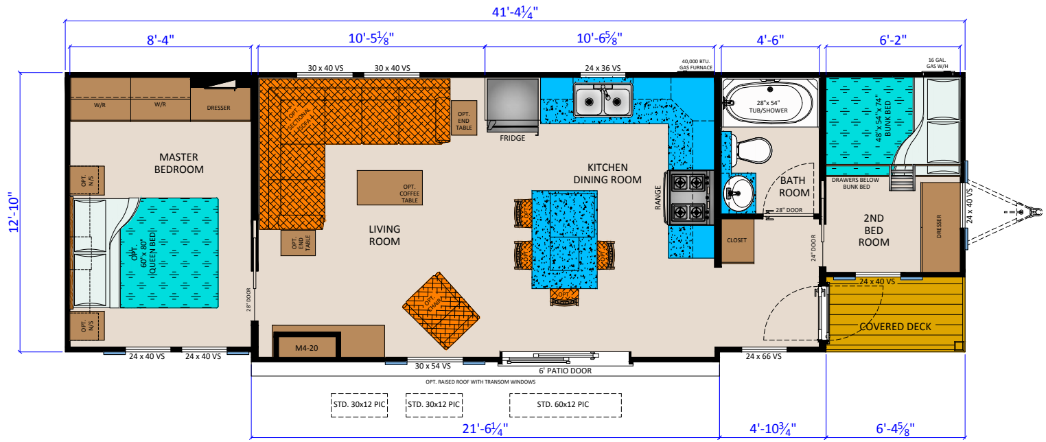
MIRABEL - 21 (M4113 2BR CK) (540 SQ.FT.)
