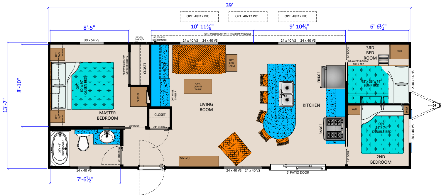
MILTON - 21 (M3914 3BR CK) (530 SQ.FT.)
