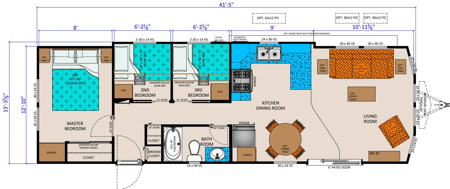
McKELLAR - 21 (M4113 3BR FL) (539 SQ.FT.)
