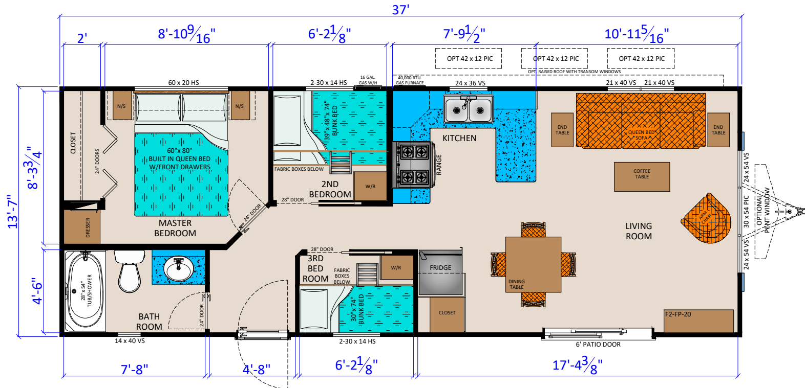
FLORENCE 21 (F3714 3BR) (502 SQ.FT.)
