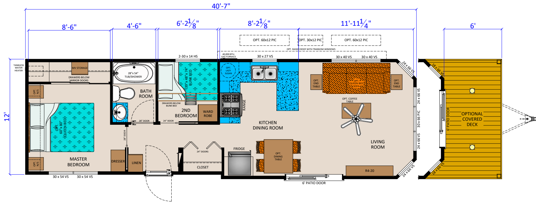
RIVERVIEW 20 (R4012 2BR FL) (493 SQ.FT.)
