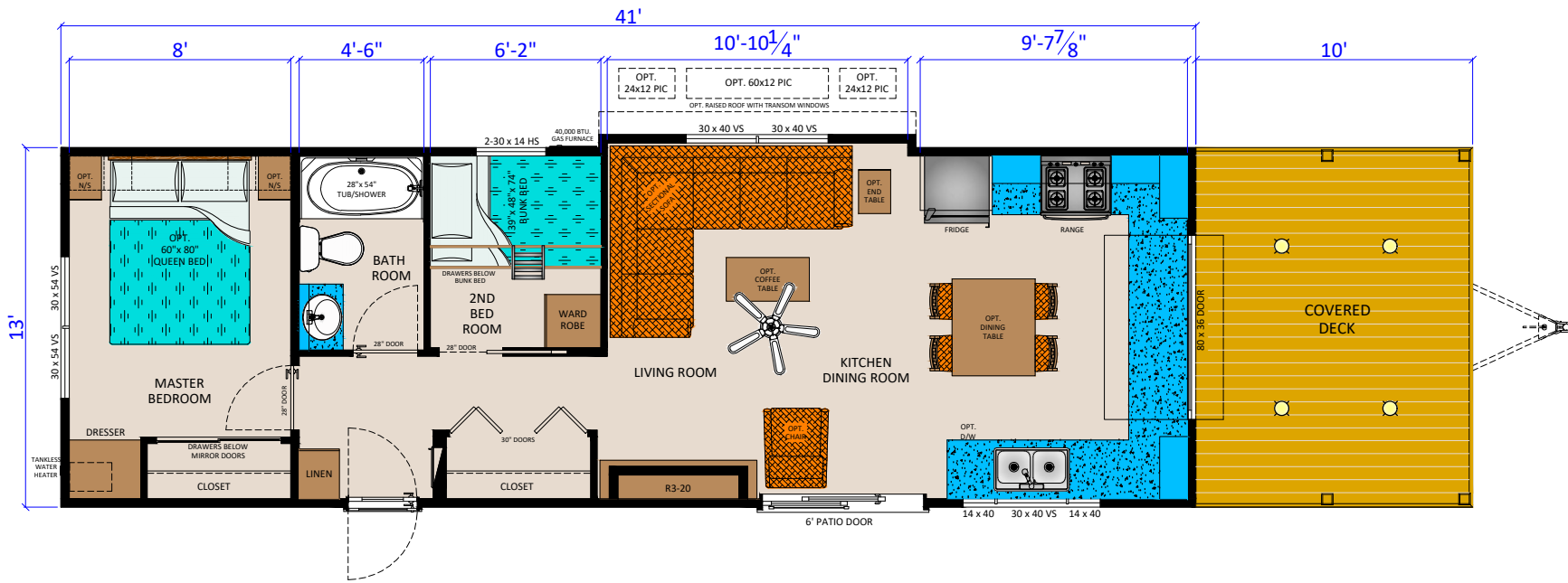
RICHIEU 20 (4113 2BR FK) (533 SQ.FT.)
