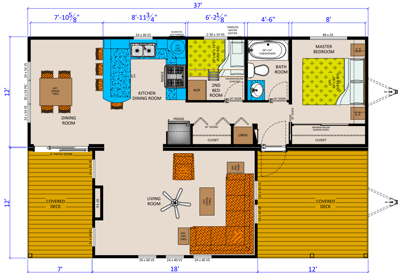
RICHAN 20 (3612 2BR FD) (444 SQ.FT.)+(216 SQ.FT.)
