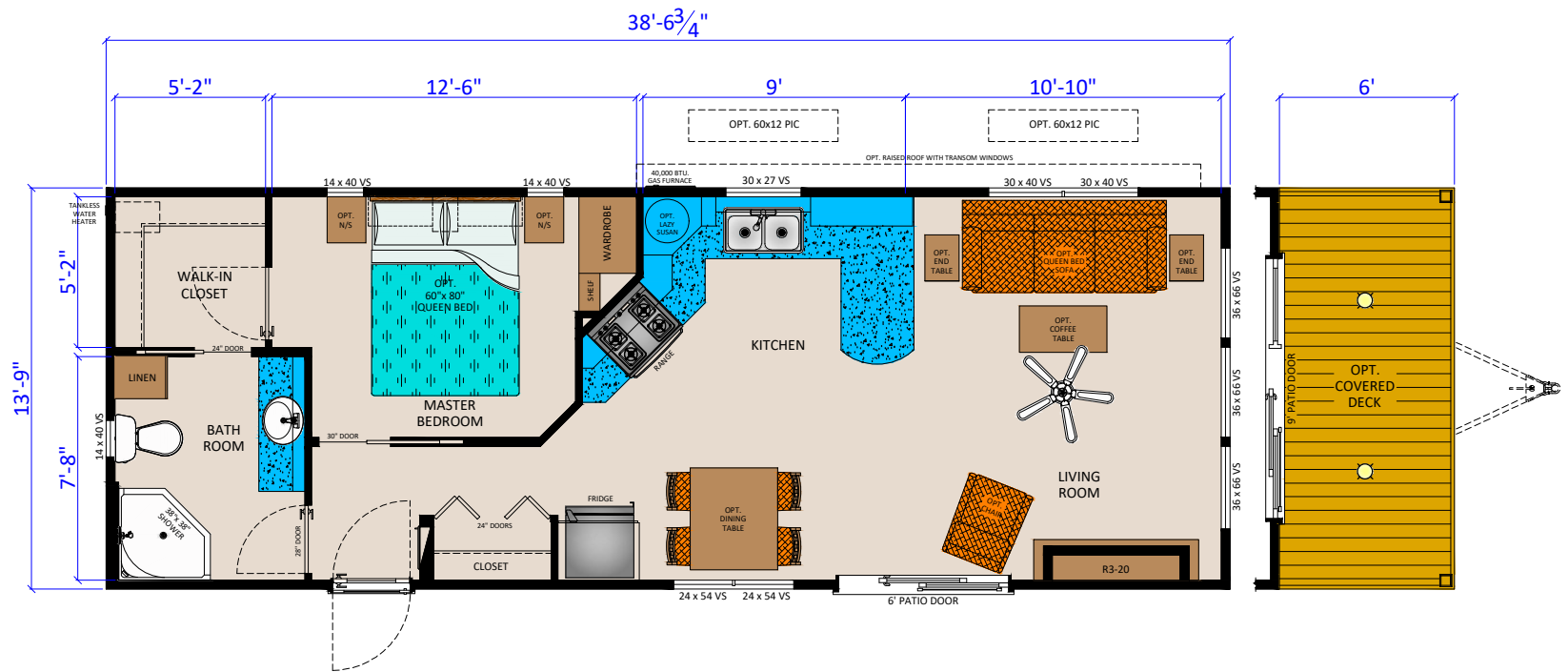
RAMSEY 20 (R3914 1BR) (540 SQ.FT.)
