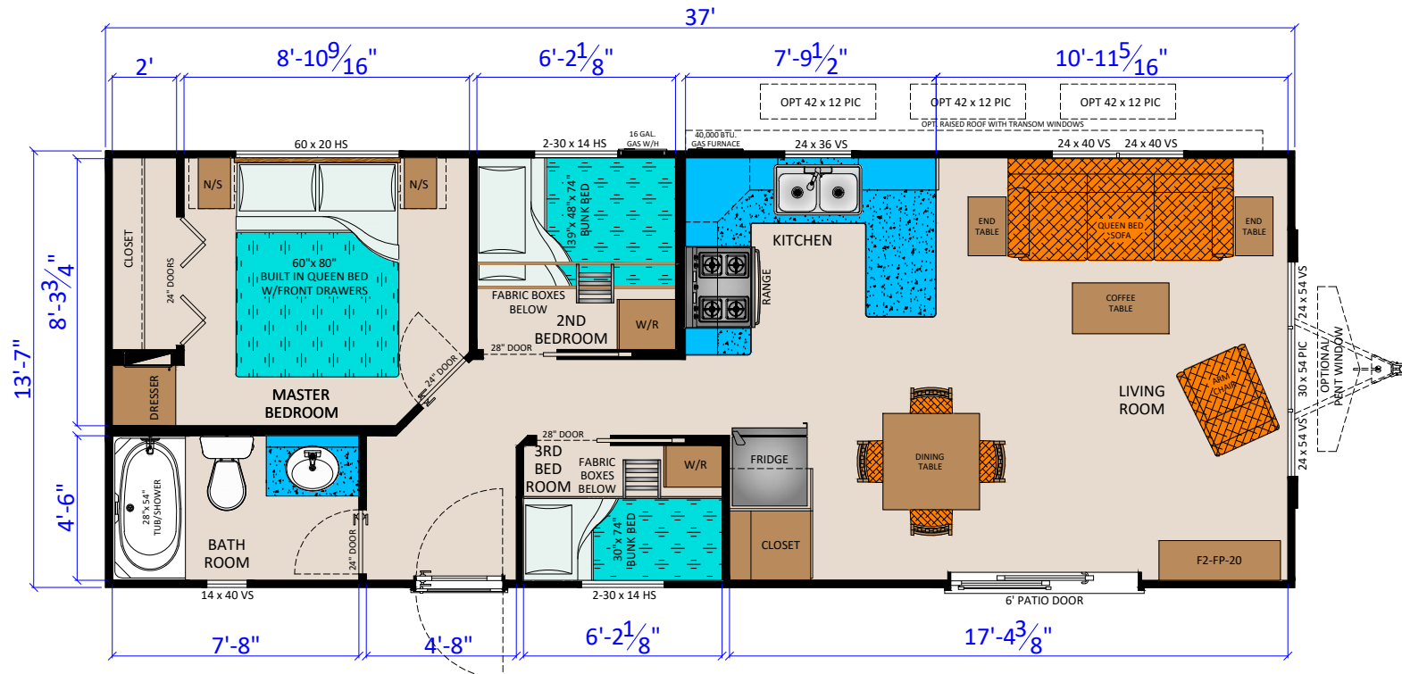
FLORENCE 20 (F3714 3BR CK) (502 SQ.FT.)
