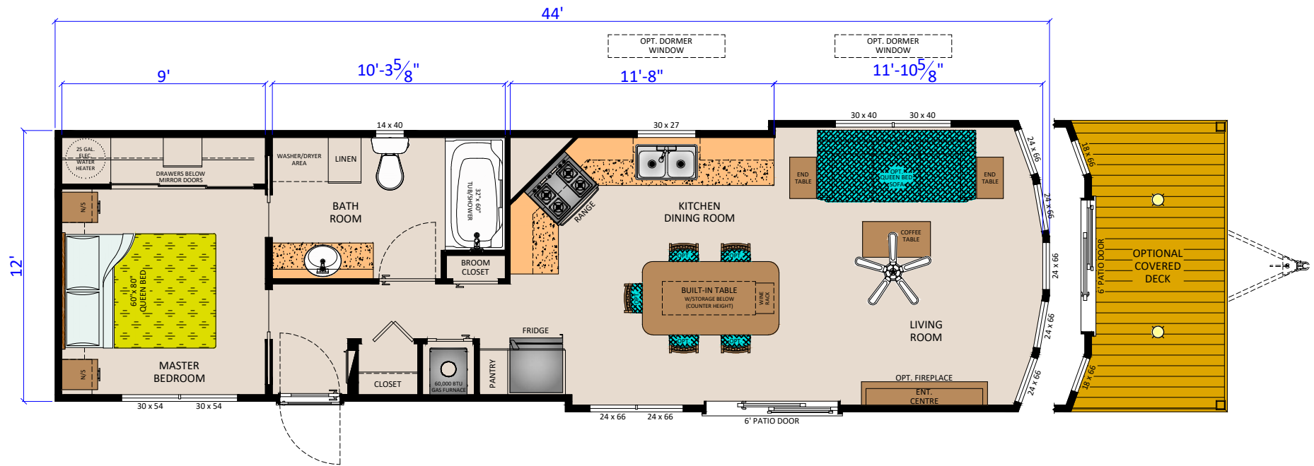
RUSTICO 1 19 (R4412 1BR FL) (537.7 SQ.FT.)
