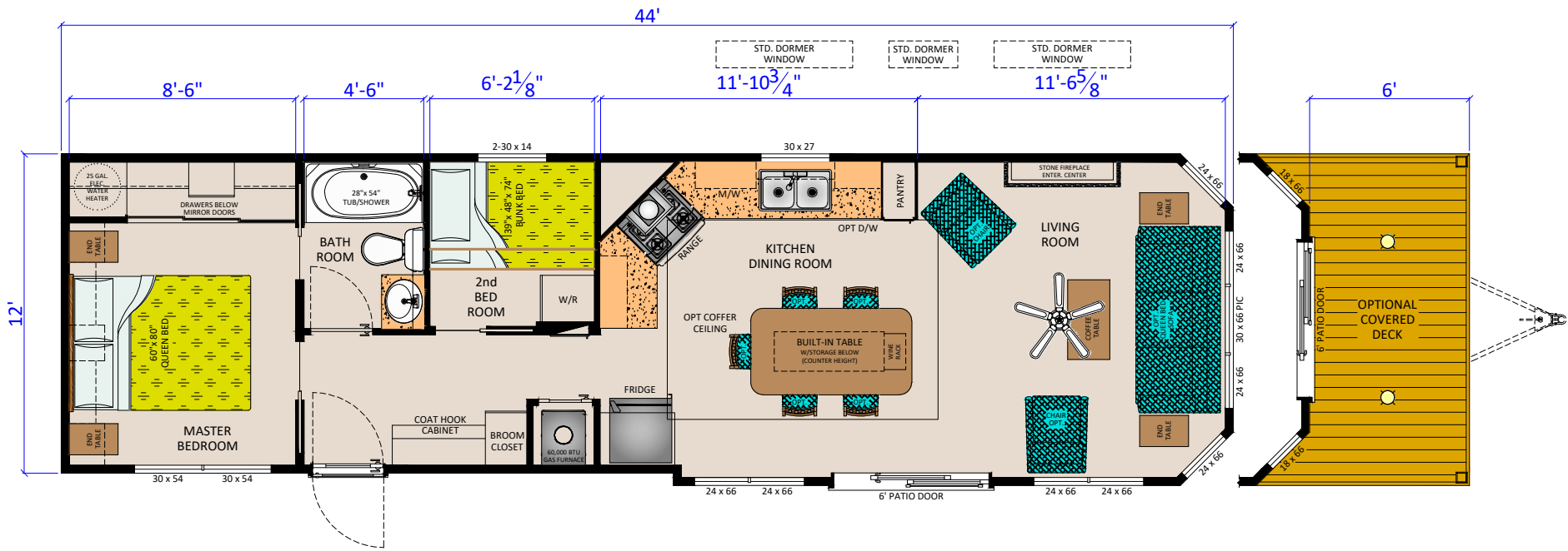
RIDGETOWN 2 19 (R4412 2BR FL) (537.7 SQ.FT.)
