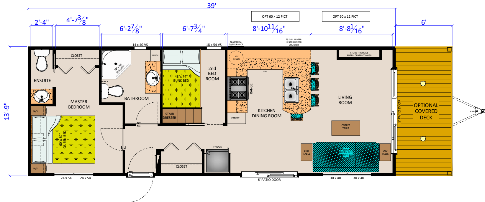
REVELSTOKE 19 (R3914 2BR FLD) (538.6 SQ.FT.)
