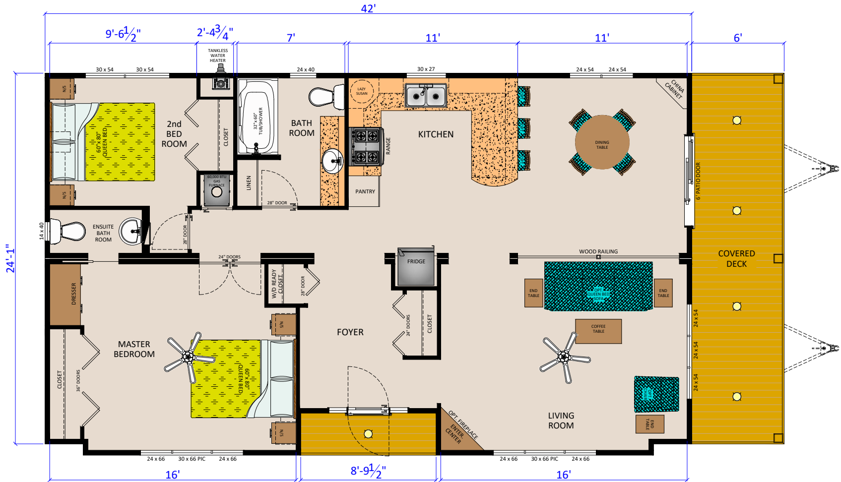
RALSTON 19 (R4224) (504 SQ.FT.)+(506.8 SQ.FT.)
