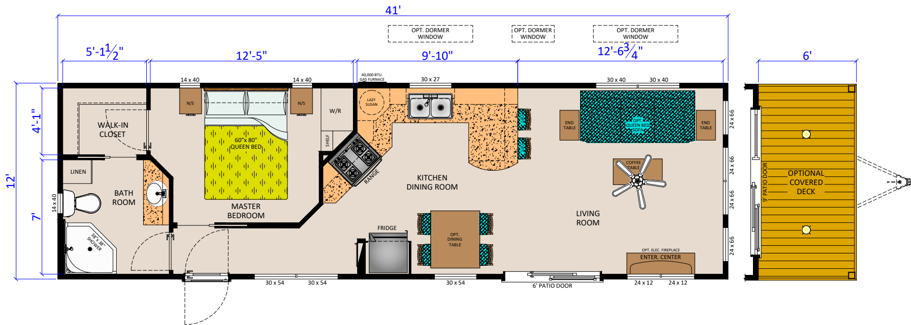
RADISSON 19 (R4012 1BR FL) (492 SQ.FT.)
