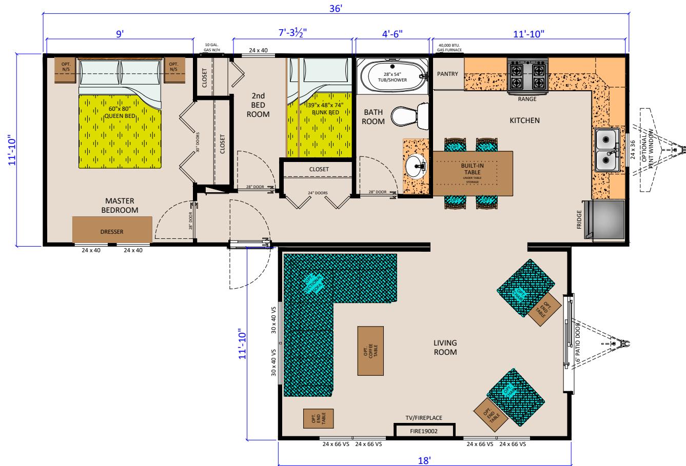
MUSKOKA - 19 (F3612 2BR FK) (426 SQ.FT.)+(213 SQ.FT.)
