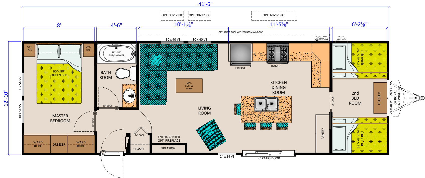
MARTENSVILLE - 19 (M4213 2BR) (533 SQ.FT.)
