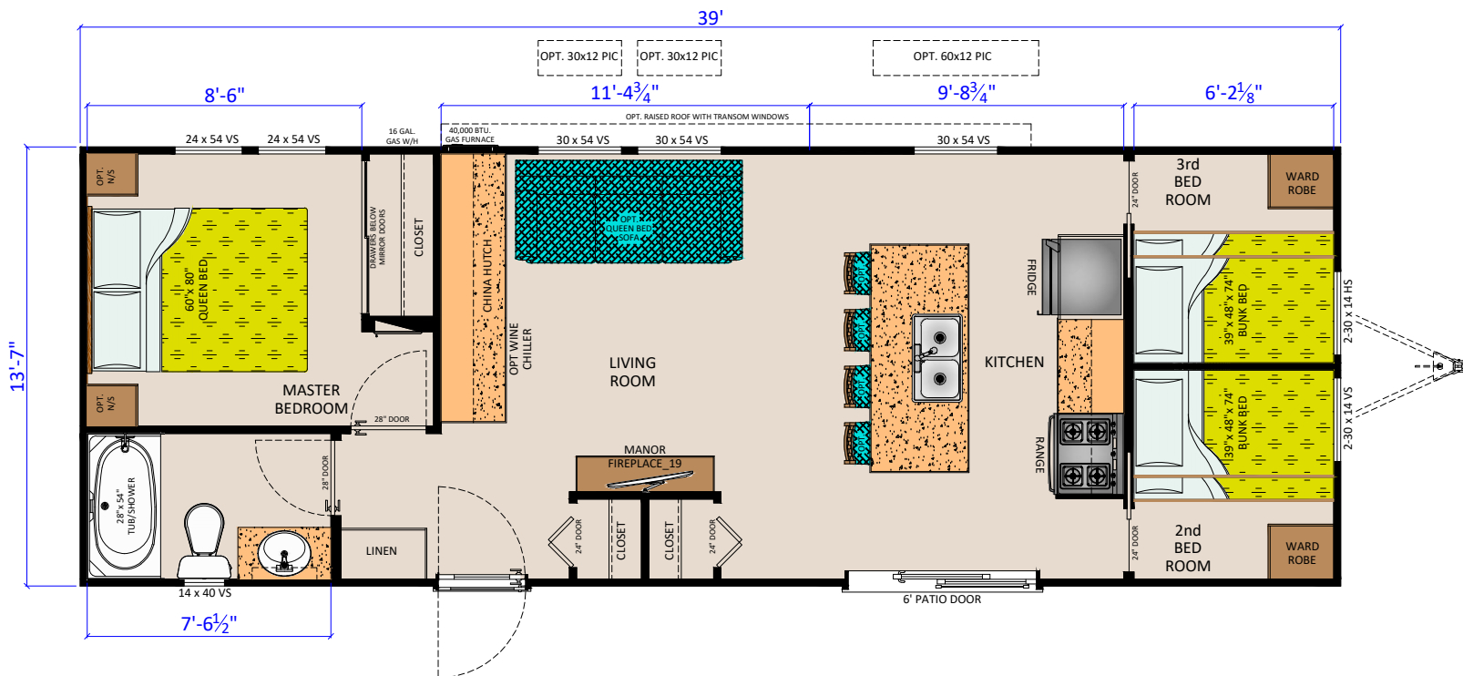
MADISON - 19 (M3914 3BR CK) (530 SQ.FT.)
