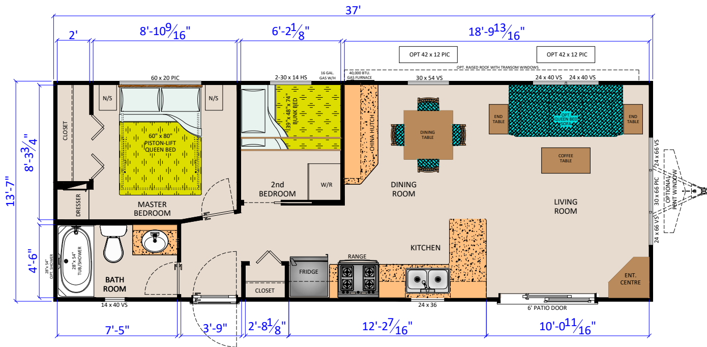
FONTHILL 19 (F3714 2BR CK) (502 SQ.FT.)
